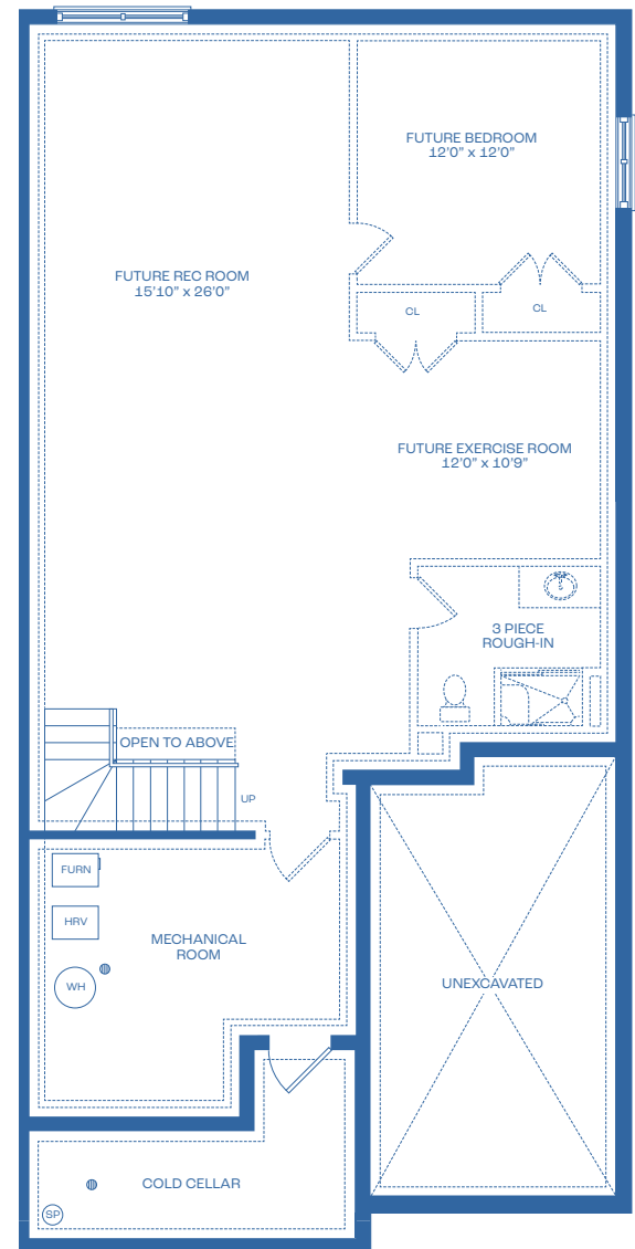
BASEMENT 1068 SQFT Excluding Mechanical Room
