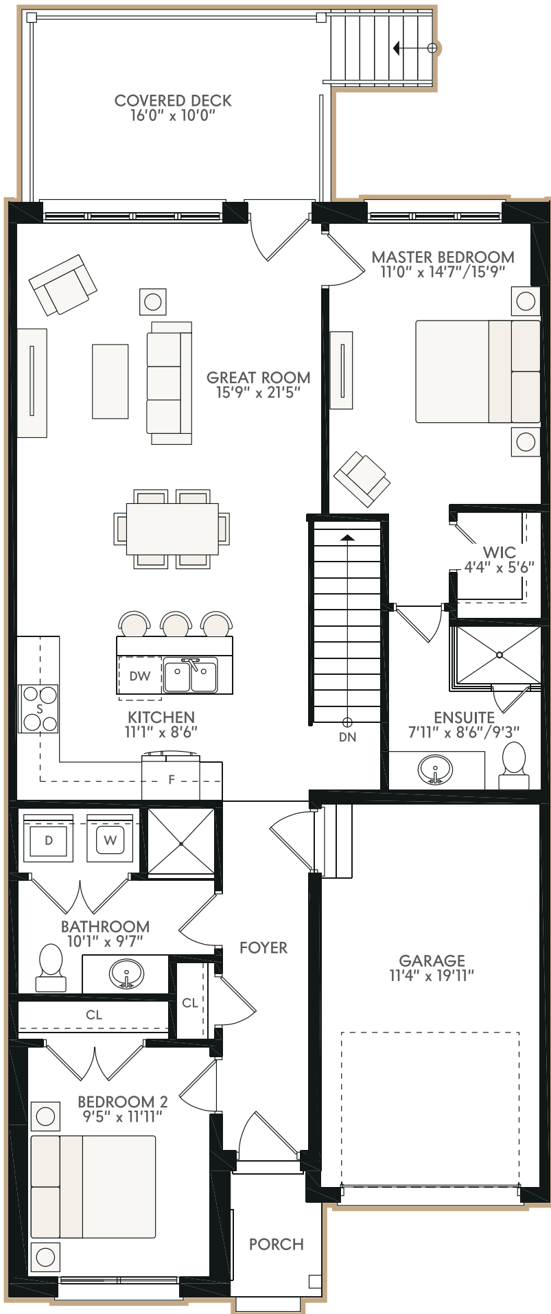
MAIN FLOOR 1254 SQFT
